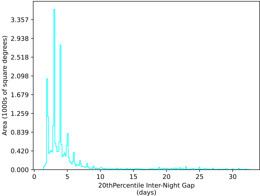
all_long_v3.4_10yrs All sky u band: 20thPercentile Inter-Night Gap
