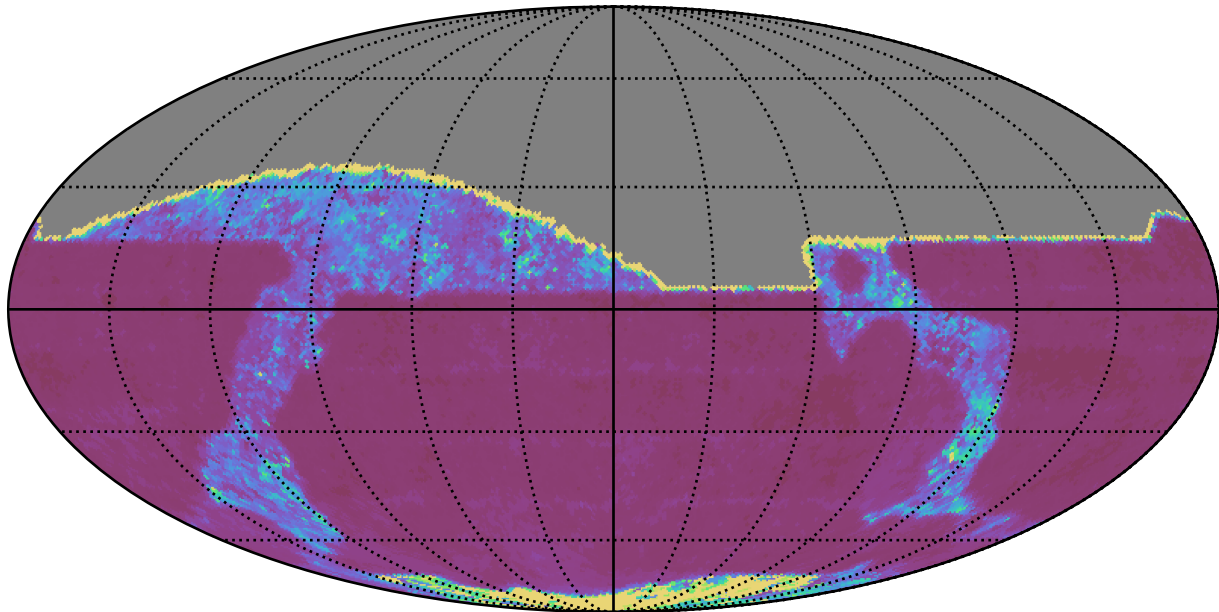
all_long_v3.4_10yrs All sky r band: 20thPercentile Inter-Night Gap
