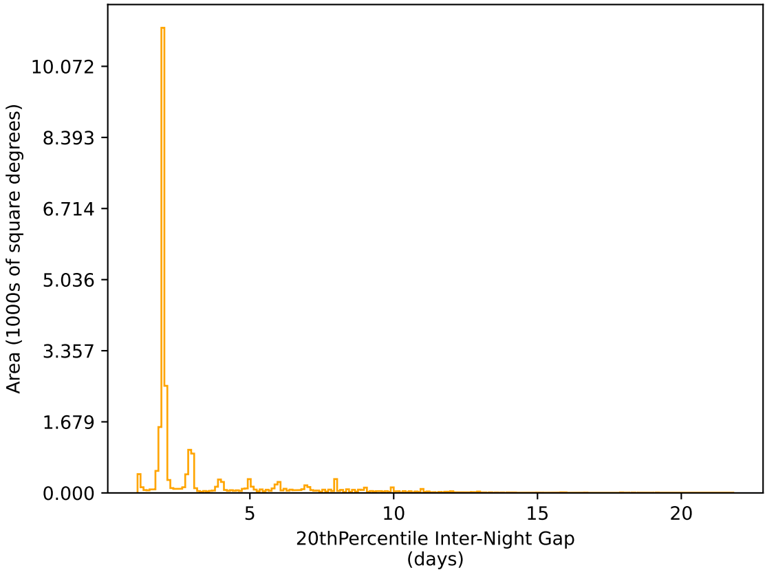
all_long_v3.4_10yrs All sky r band: 20thPercentile Inter-Night Gap
