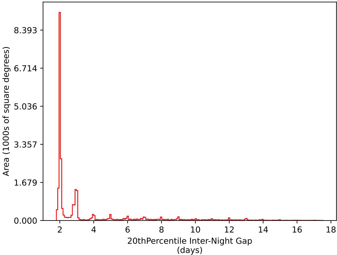
all_long_v3.4_10yrs All sky i band: 20thPercentile Inter-Night Gap
