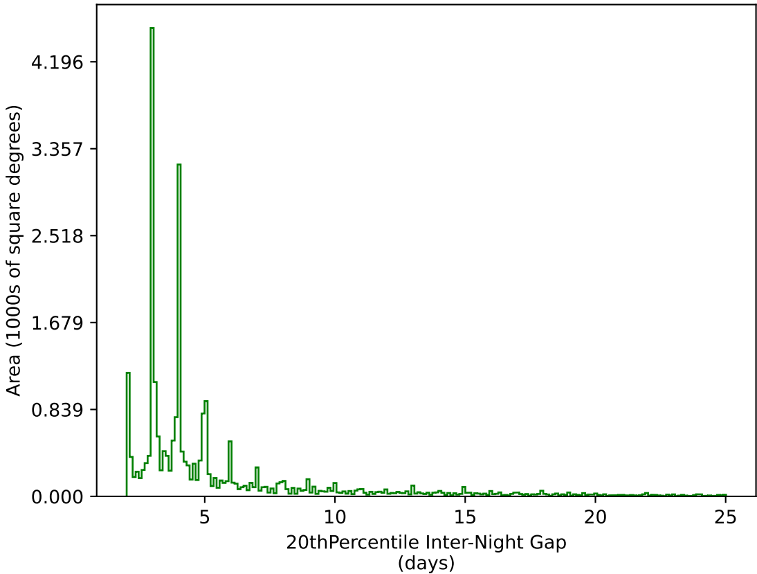
all_long_v3.4_10yrs All sky g band: 20thPercentile Inter-Night Gap
