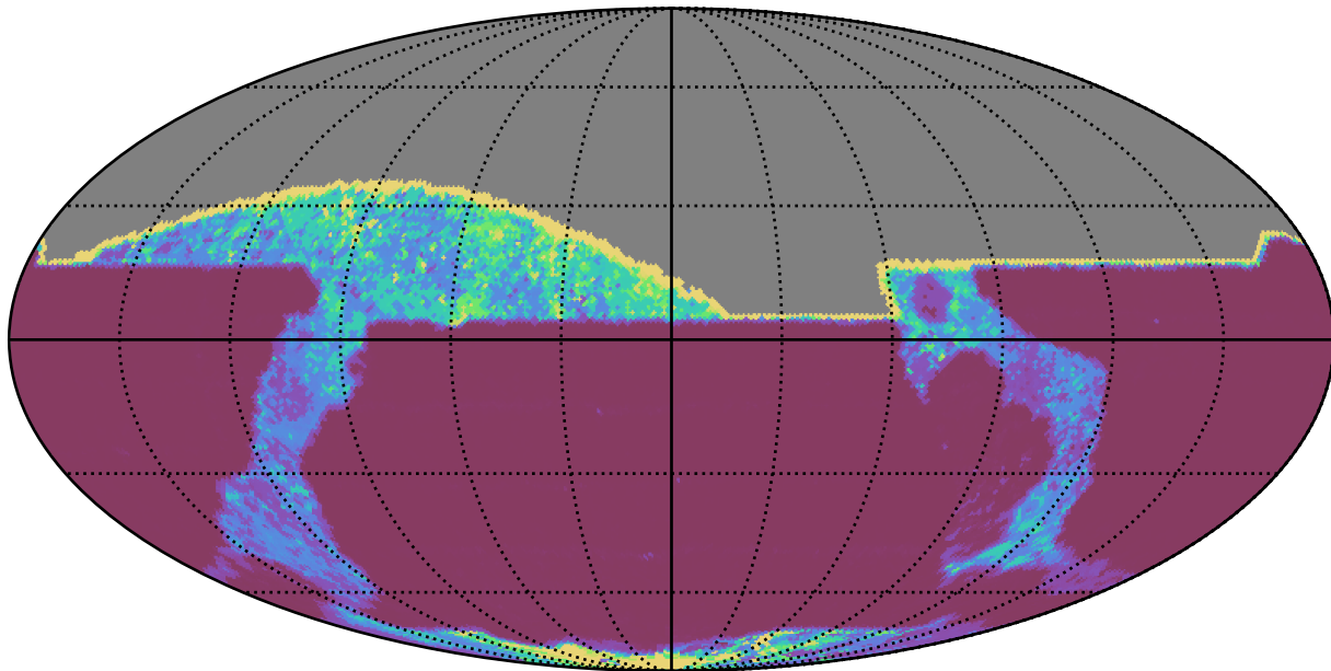
all_long_v3.4_10yrs All sky all bands: 20thPercentile Inter-Night Gap
