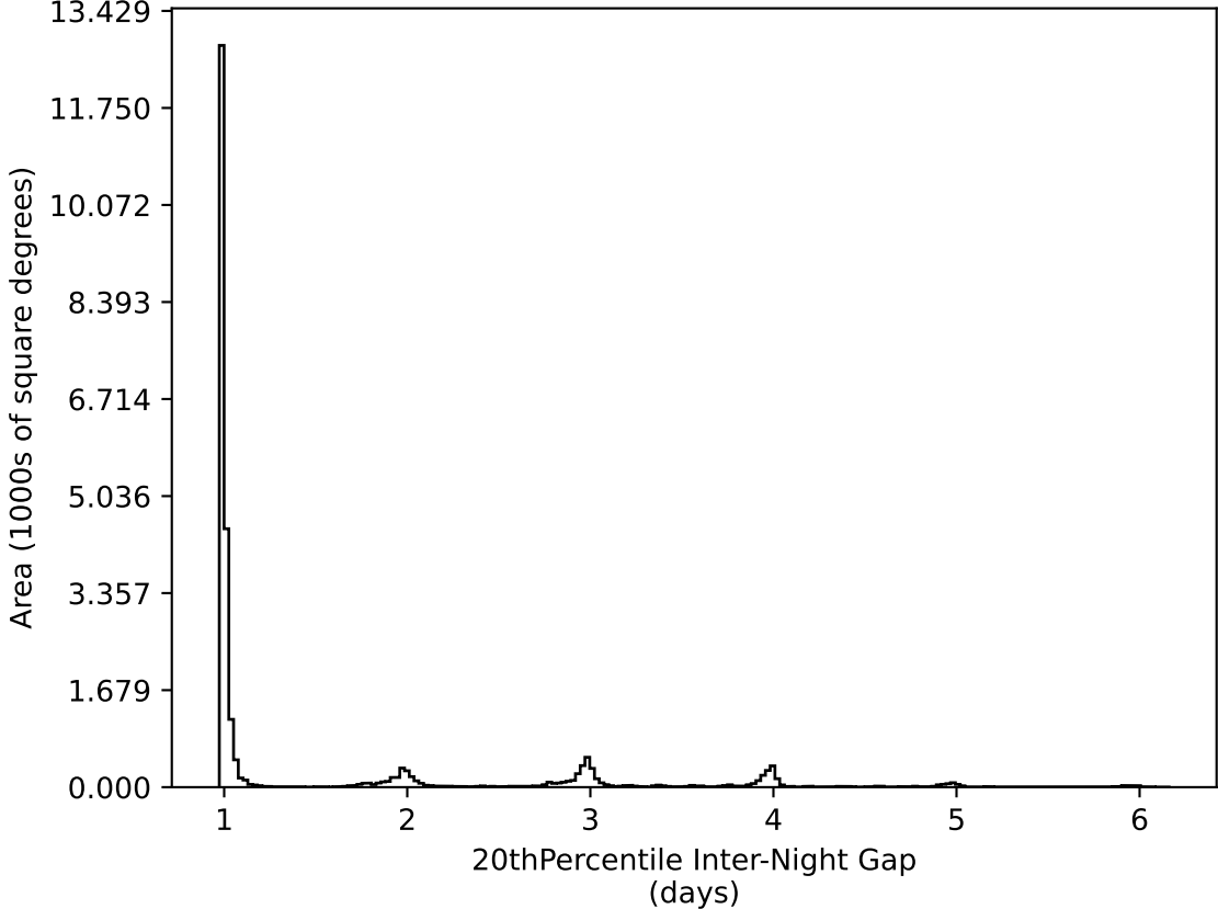
all_long_v3.4_10yrs All sky all bands: 20thPercentile Inter-Night Gap
