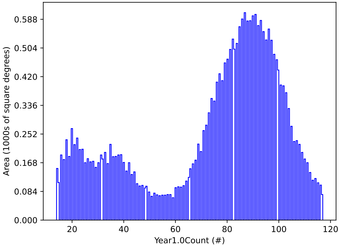
all_long_v3.4_10yrs night < 365.25: Year1.0Count
