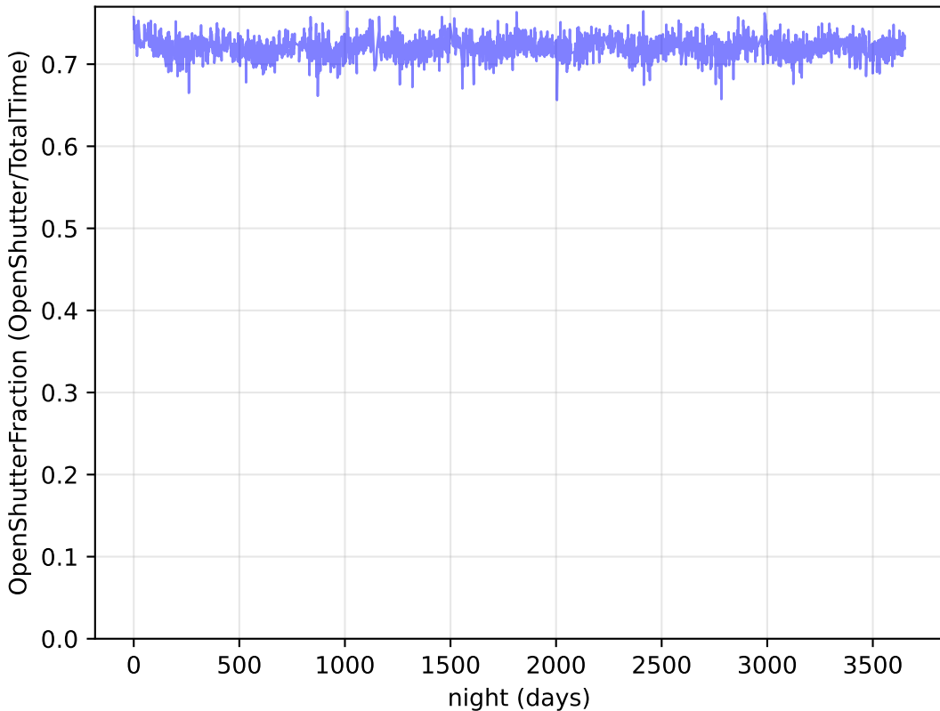
all_long_v3.4_10yrs : OpenShutterFraction
