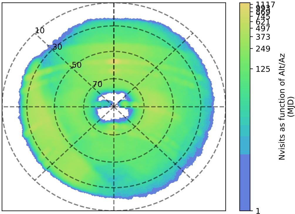
all_long_v3.4_10yrs g: Nvisits as function of Alt/Az
