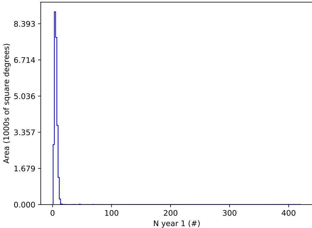
all_long_v3.4_10yrs u and night < 365: N year 1
