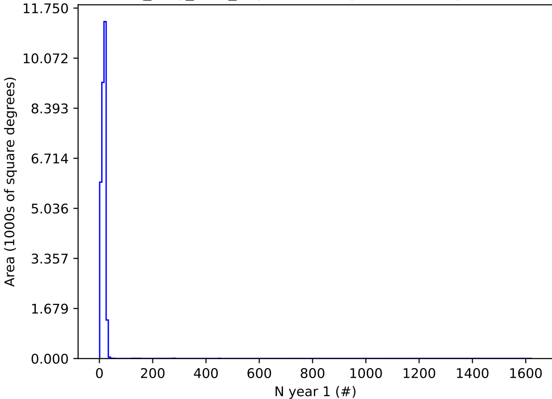
all_long_v3.4_10yrs r and night < 365: N year 1
