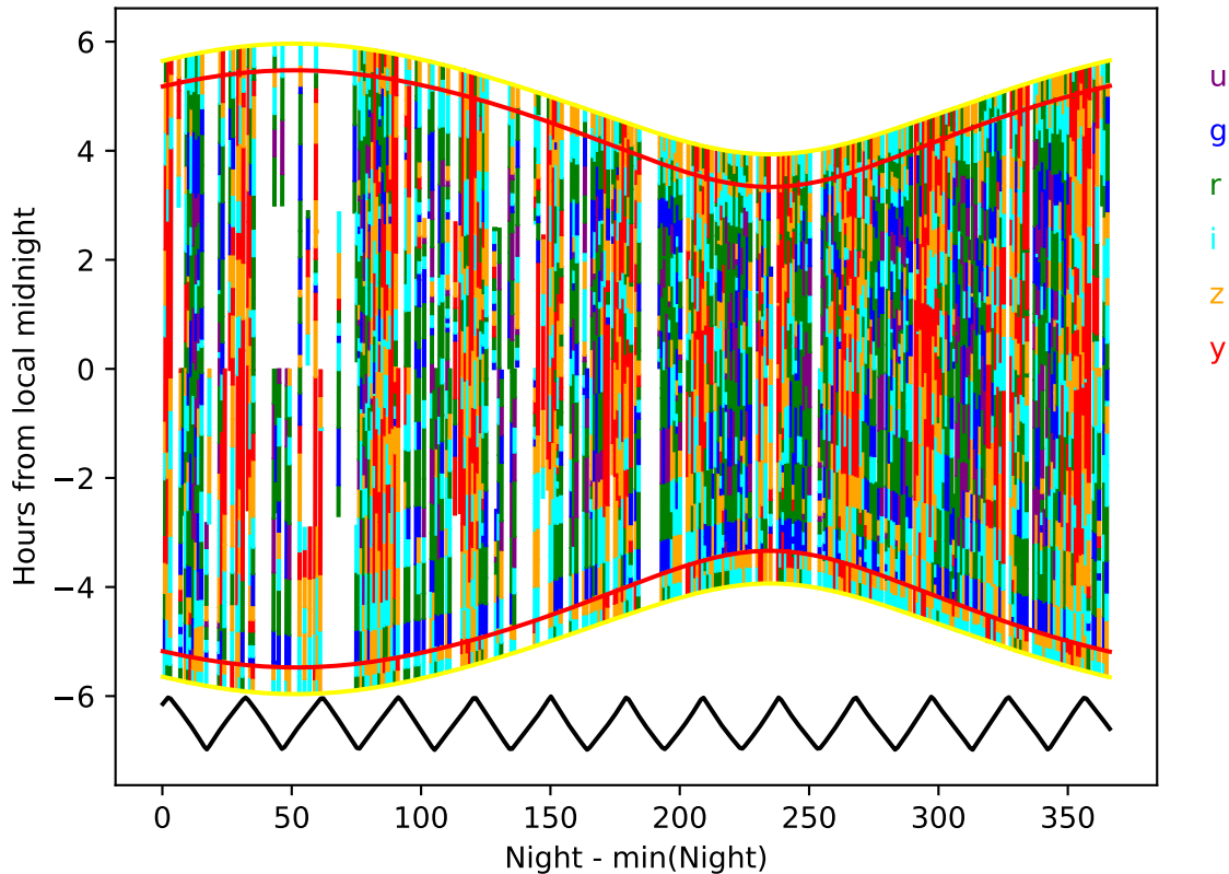
all_long_v3.4_10yrs year 9-10: Hourglass
