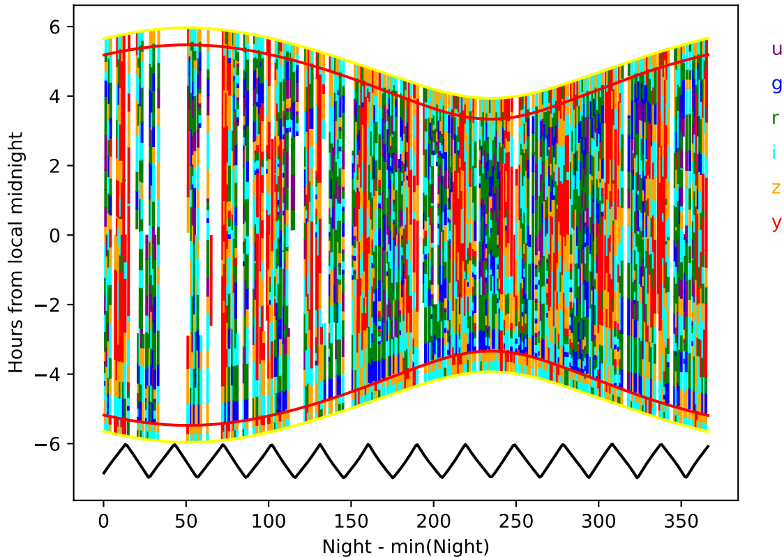
all_long_v3.4_10yrs year 8-9: Hourglass
