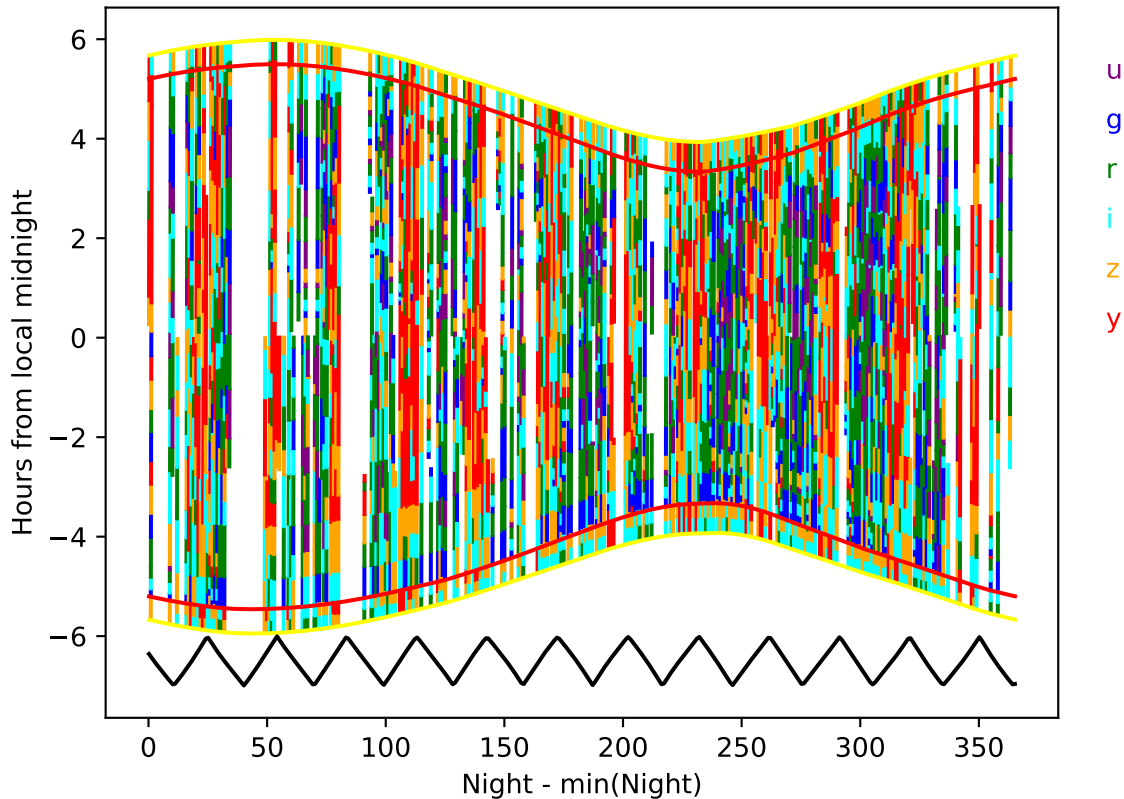
all_long_v3.4_10yrs year 4-5: Hourglass
