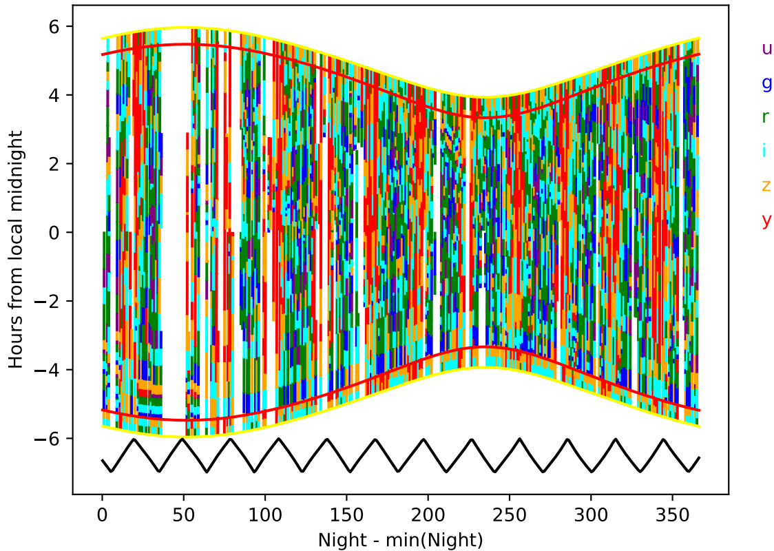
all_long_v3.4_10yrs year 2-3: Hourglass
