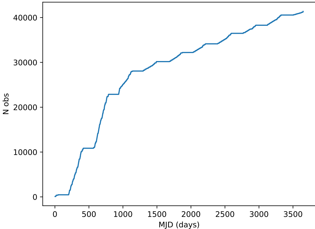
all_long_v3.4_10yrs note like DD:COSMOS%: Cumulative
