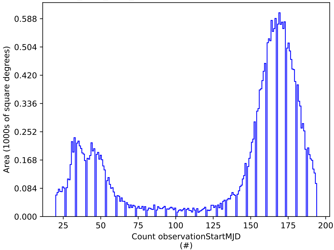
all_long_v3.4_10yrs z: Count observationStartMJD
