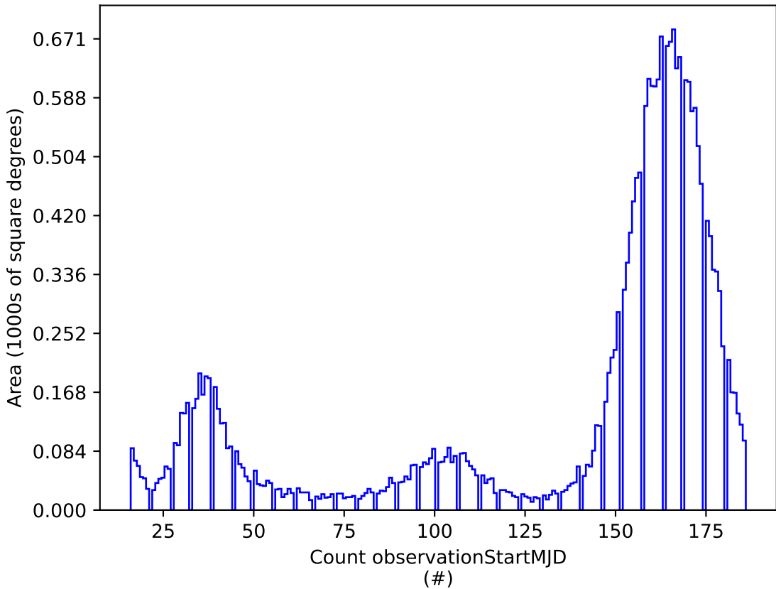
all_long_v3.4_10yrs y: Count observationStartMJD
