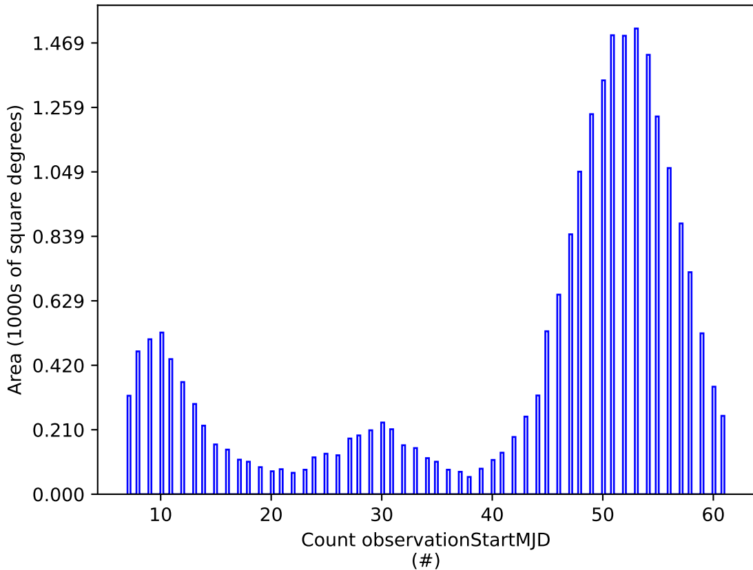
all_long_v3.4_10yrs u: Count observationStartMJD
