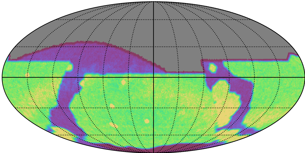
all_long_v3.4_10yrs r: Count observationStartMJD
