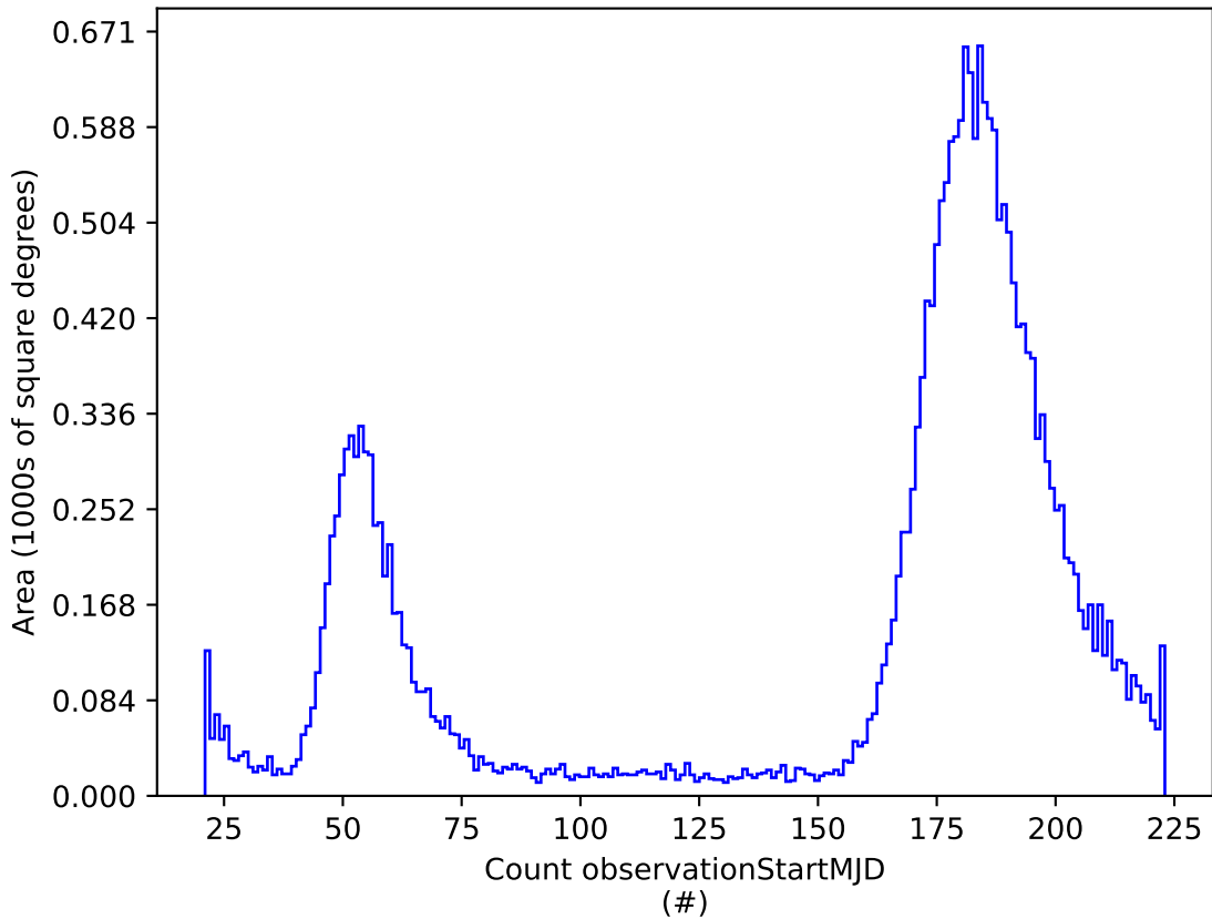
all_long_v3.4_10yrs r: Count observationStartMJD
