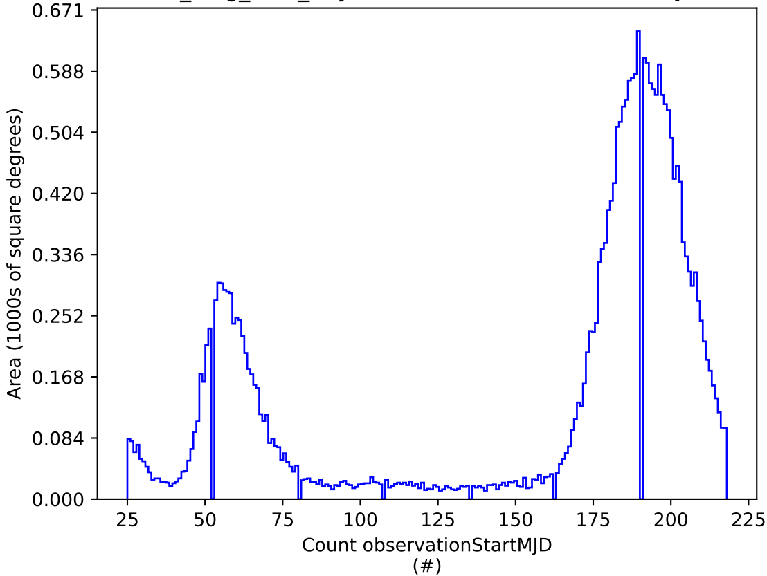
all_long_v3.4_10yrs i: Count observationStartMJD
