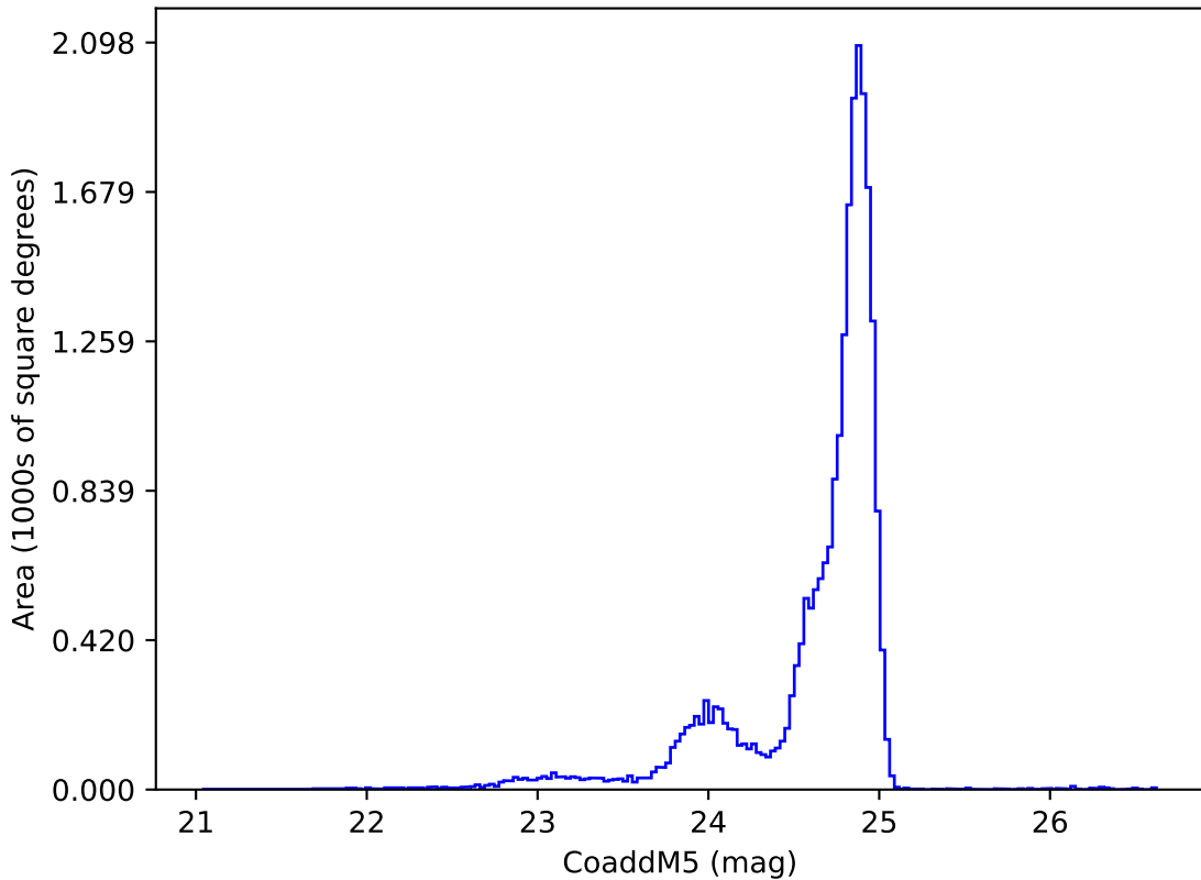
all_long_v3.4_10yrs y: CoaddM5
