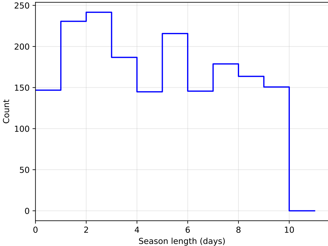
all_long_v3.4_10yrs DD:WFD all bands: SeasonLength
