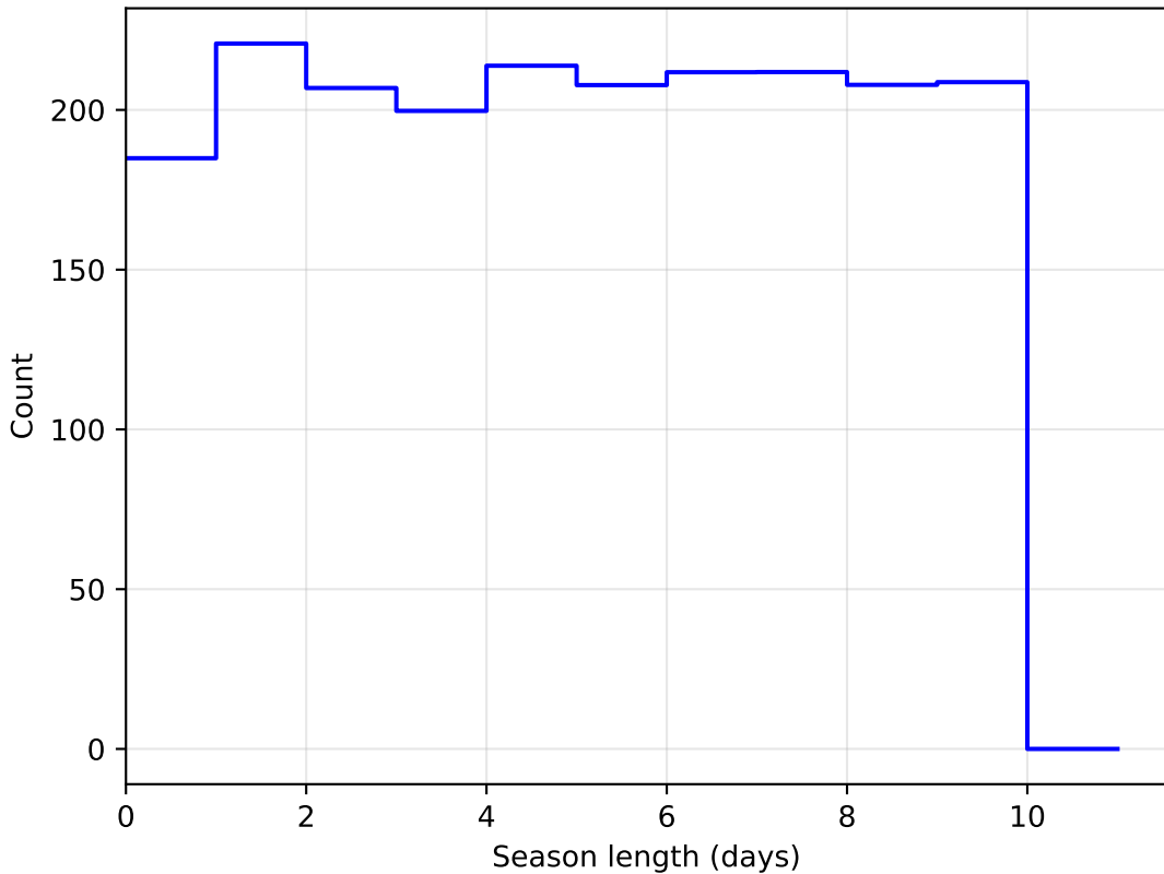
all_long_v3.4_10yrs DD:ELAISS1 all bands: SeasonLength
