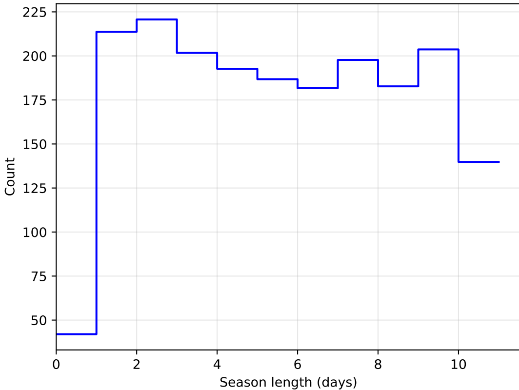
all_long_v3.4_10yrs DD: COSMOS all bands: SeasonLength
