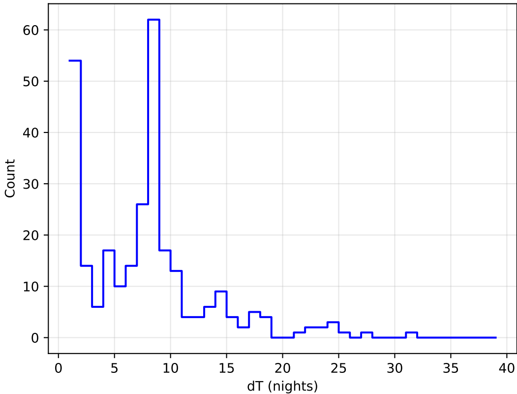
all_long_v3.4_10yrs all bands: DD:XMM_LSS Delta Nights Histogram
