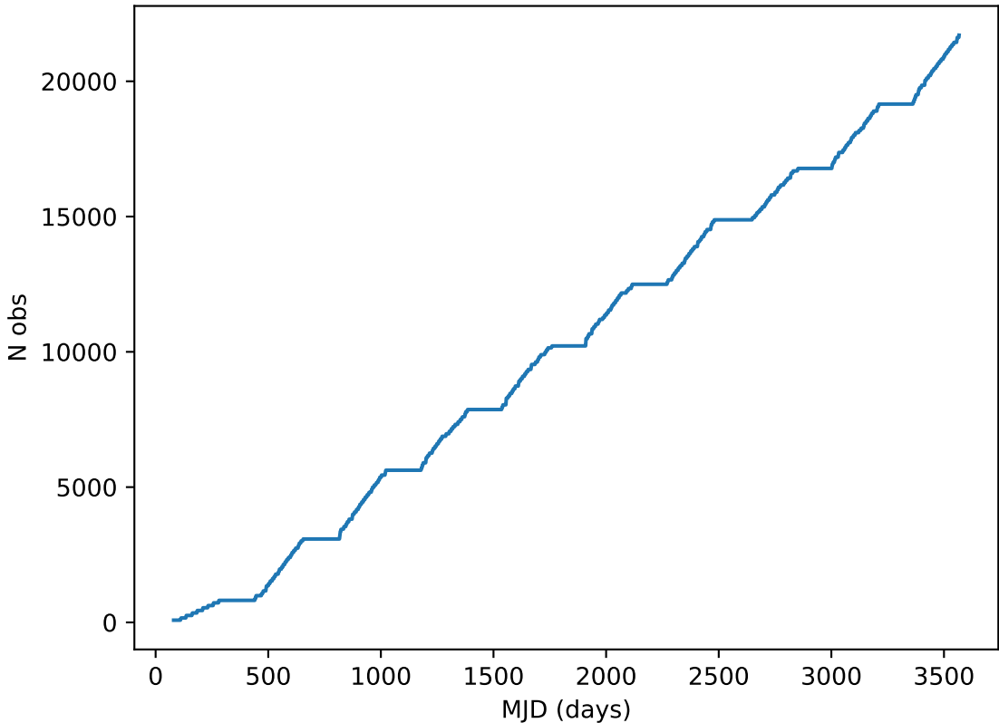
all_long_v3.4_10yrs all bands: DD:XMM_LSS Cumulative NVisits
