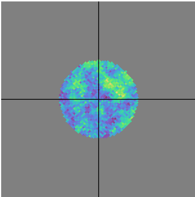
all_long_v3.4_10yrs all bands: DD:WFD NVisits
