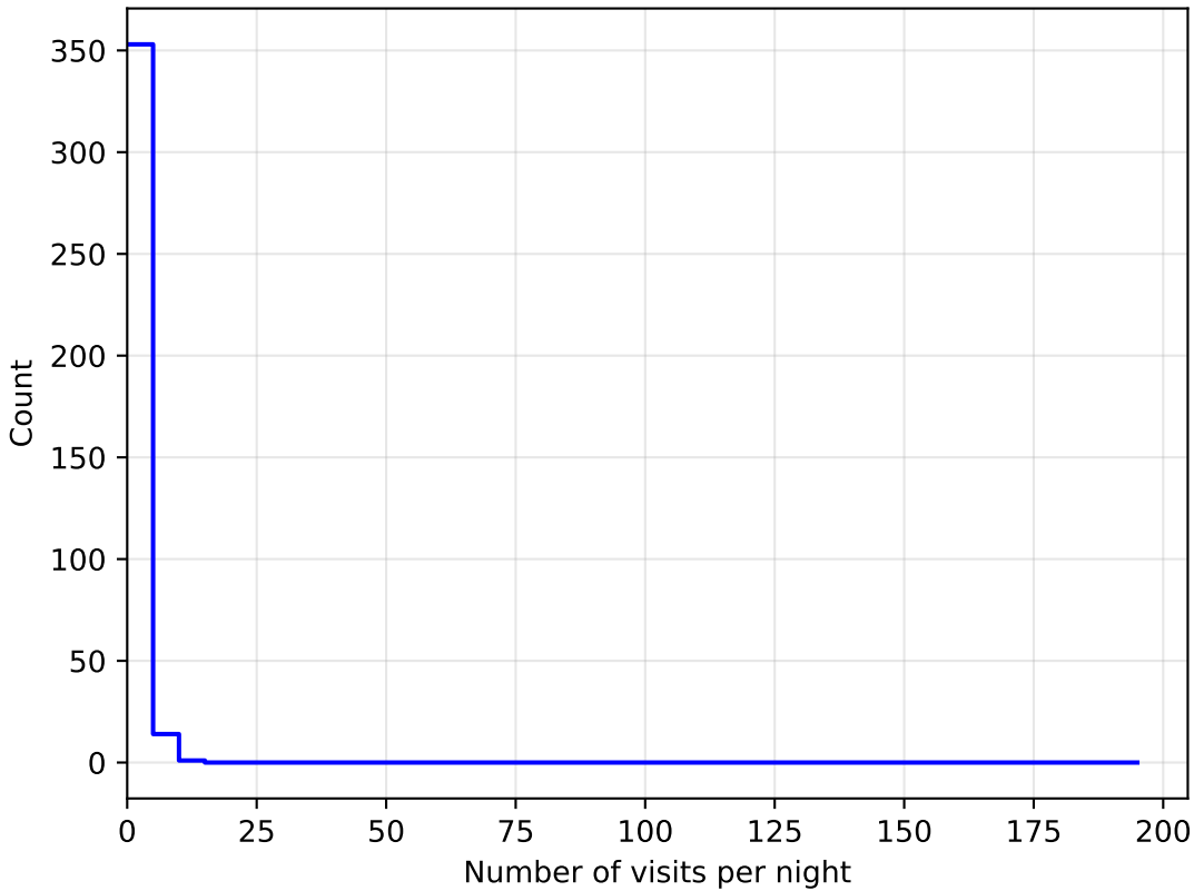
all_long_v3.4_10yrs all bands: DD:WFD NVisitsPerNight
