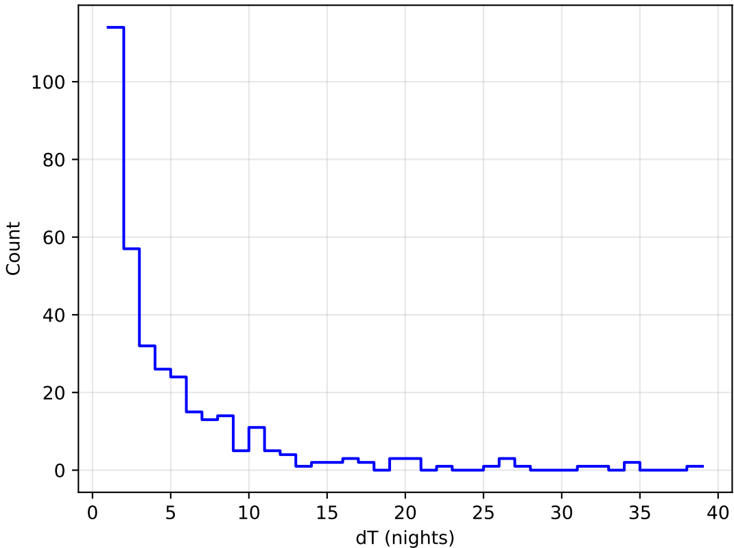
all_long_v3.4_10yrs all bands: DD:WFD Delta Nights Histogram
