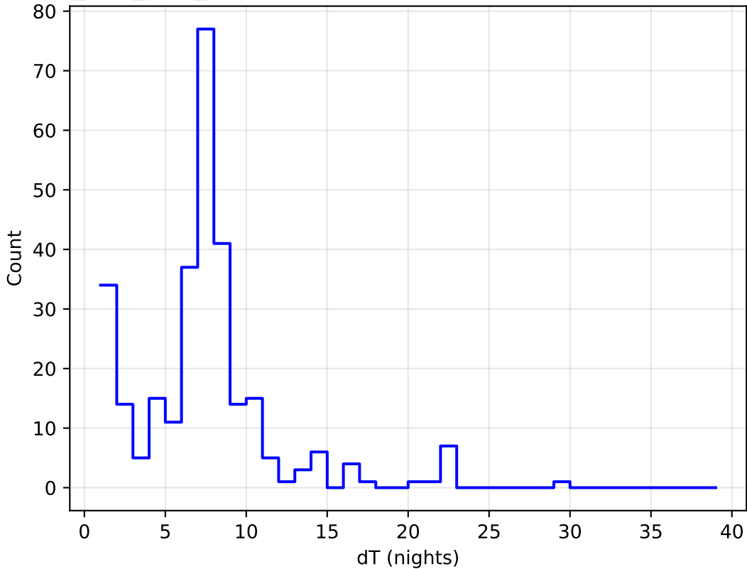
all_long_v3.4_10yrs all bands: DD:EDFS Delta Nights Histogram
