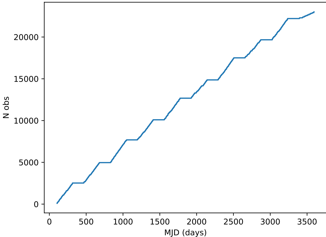
all_long_v3.4_10yrs all bands: DD:EDFS Cumulative NVisits
