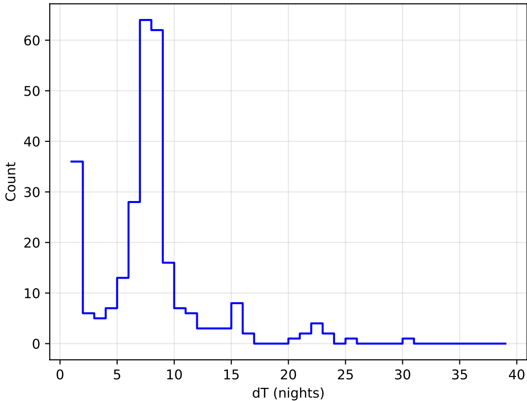
all_long_v3.4_10yrs all bands: DD:ECDFS Delta Nights Histogram
