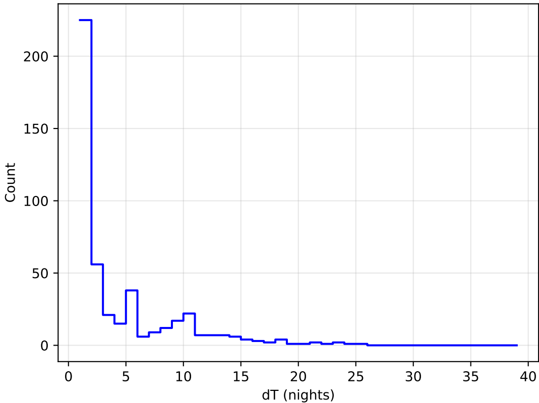
all_long_v3.4_10yrs all bands: DD: COSMOS Delta Nights Histogram
